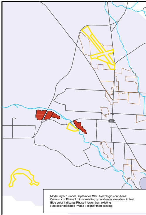
Change in Groundwater Elevation from No Project to Phase I Conditions
