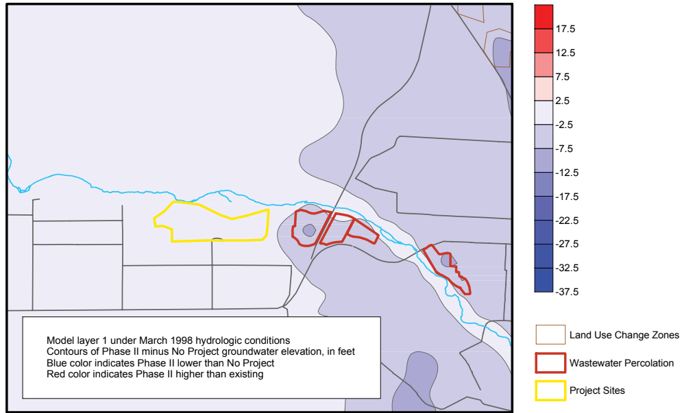
A. Change in Groundwater Elevation from No Project to Phase II Conditions
