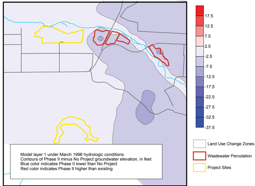
A. Change in Groundwater Elevation from No Project to Phase II Conditions
