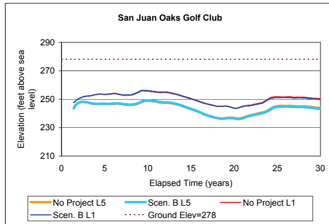
A. Change in Groundwater Elevation from No Project to Phase II Conditions
