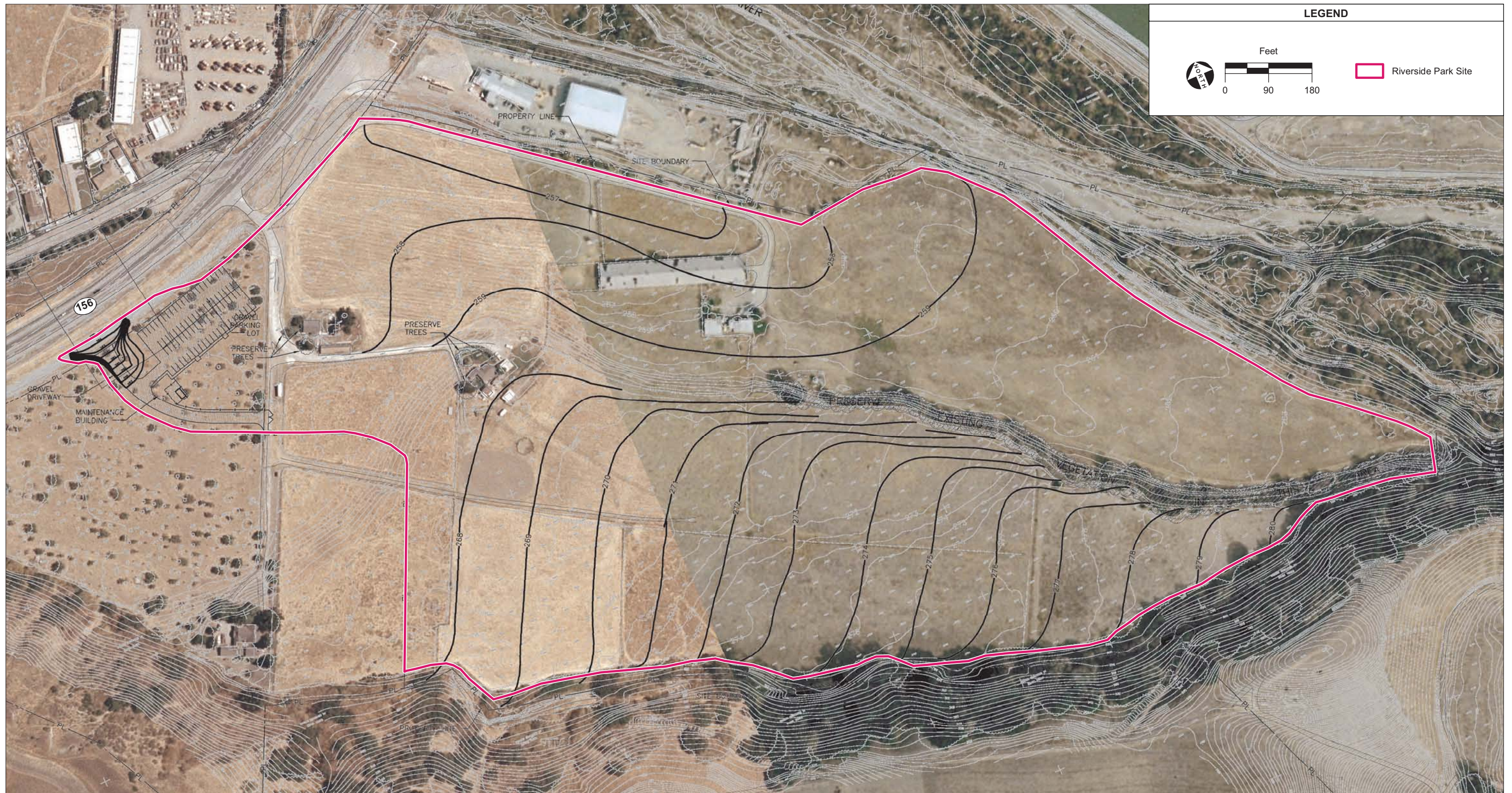
Figure 3-5 Site 3 - Riverside Park Layout Plan
