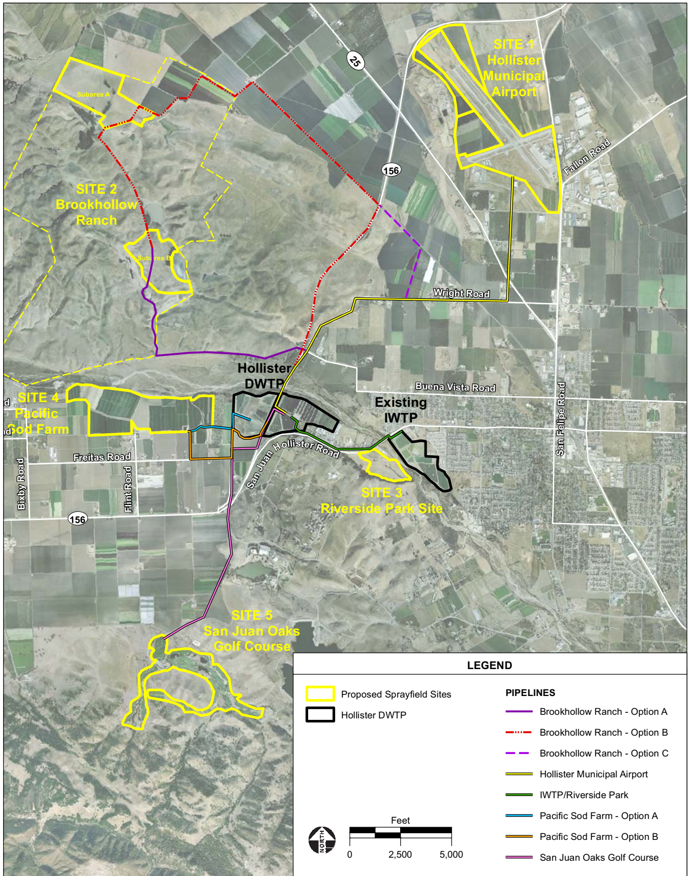
Figure 3-2 Proposed Reclamation Sites and Pipeline Locations
